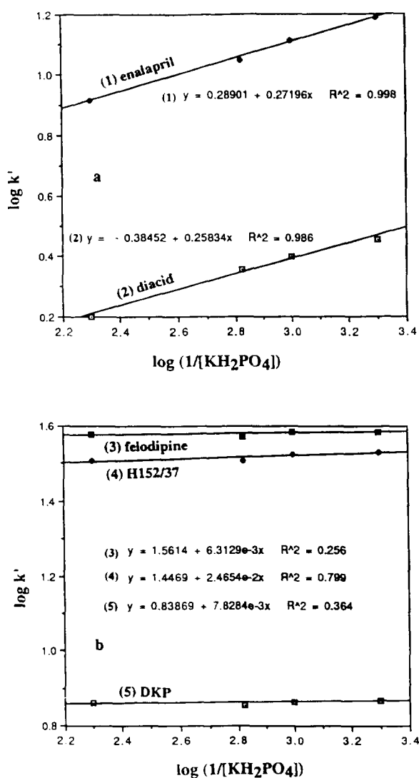
Fig. 6. Plots of \log k' vs. \log (1/[KH_2PO_4]) .
